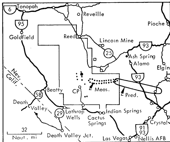
Fig. 4. Fallout from the Morgan shot fired on October 7, 1957, from a balloon at 500 ft. The solid line shows the predicted fallout pattern; the dotted line shows the actual fallout pattern. (From Ref. 2.)
